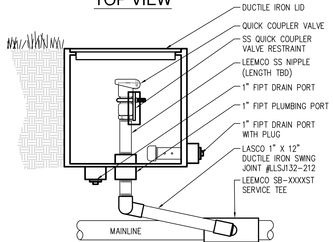
SIDE VIEW
